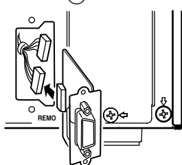
RS-422A REMOTE
